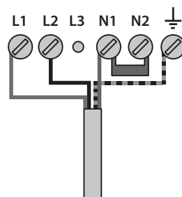
4 - Burner 2x 230/400 V
